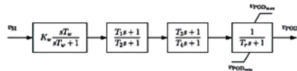
Fig. 6. Block design of POD
